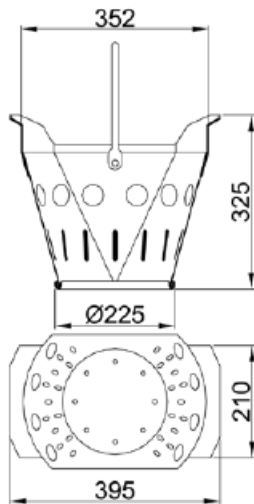
Figure 3: Oval basket, type D-1 (low)
