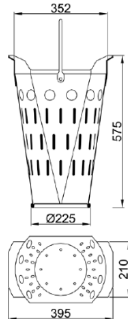
Figure 4: Oval basket, type C-3 (high)
