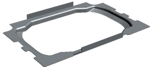
Figure 2: Adapter for LK curb-and-road drain inlet
